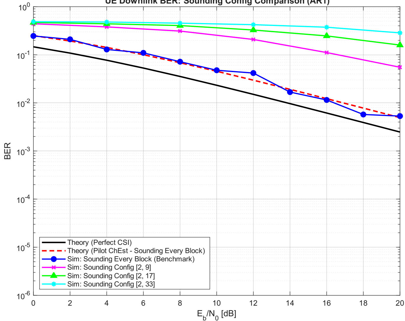
UE Downlink BER: Sounding Config Comparison (AR1)
